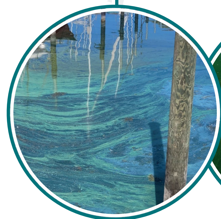
Microcystis sp.
