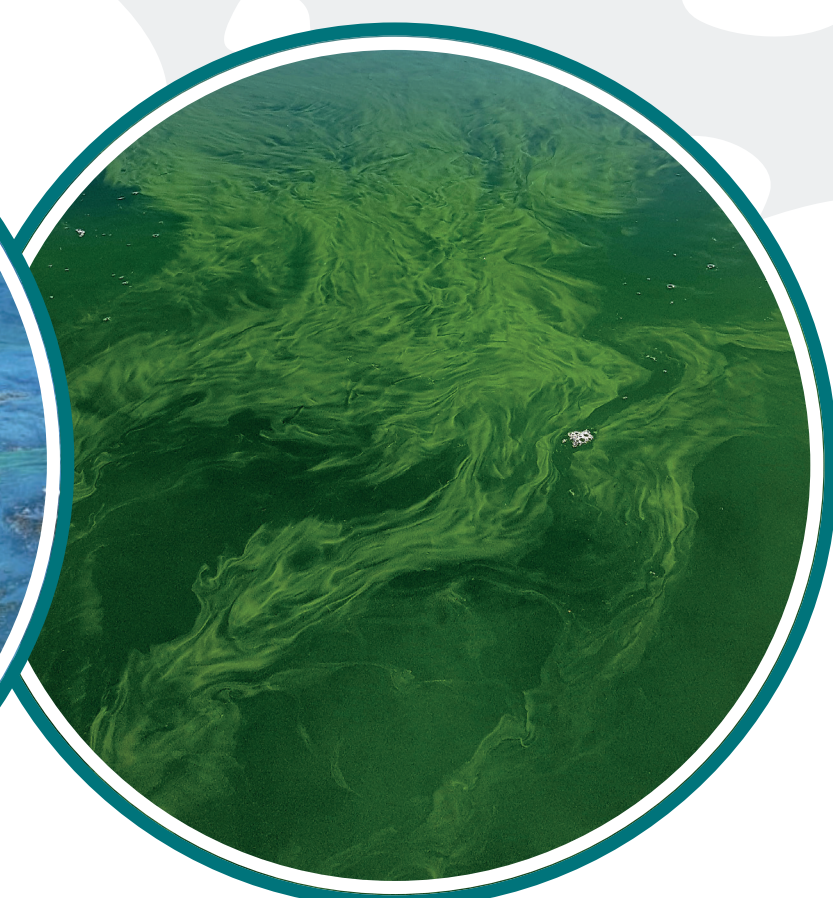
Woronichinia naegeliana
